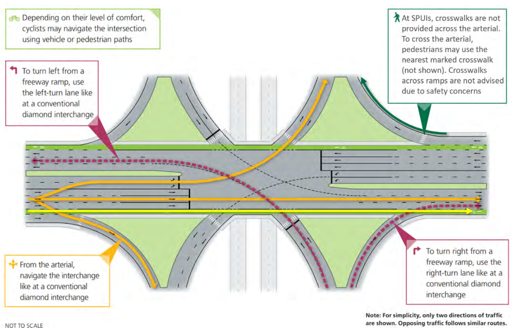
Figure 5.21: Single-point urban interchange. Source: Virginia Department of Transportation; Some additional bike and pedestrian information overlaid by Nelson\Nygaard
